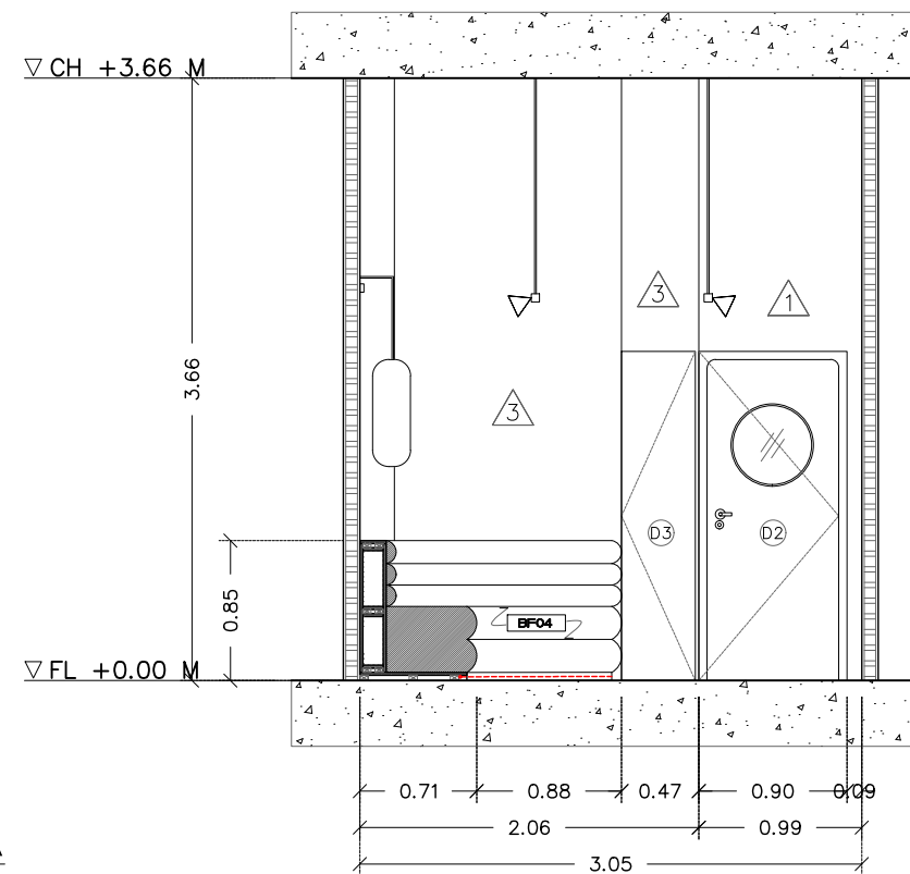
ELEVATION A SCALE 1:50
