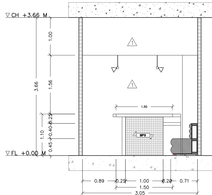
ELEVATION E SCALE 1 : 50
